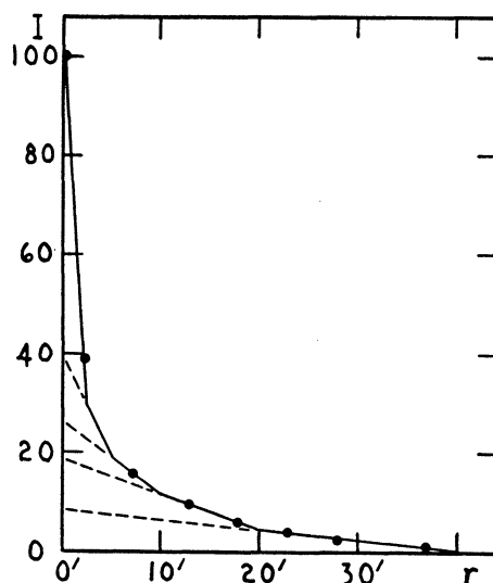
Figure 4. Surface brightness in the spiral galaxy, M33, as represented by straight sections. The dots represent the observations of S. Patterson.
