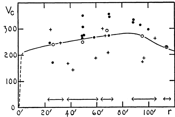
Figure 1. Circular velocity in the Andromeda Nebula in km/sec. Dots: observations on north following side. Crosses: observations on south preceding side. Circles: normal points. Curve: computed under assumption of identical mass and light distributions.
