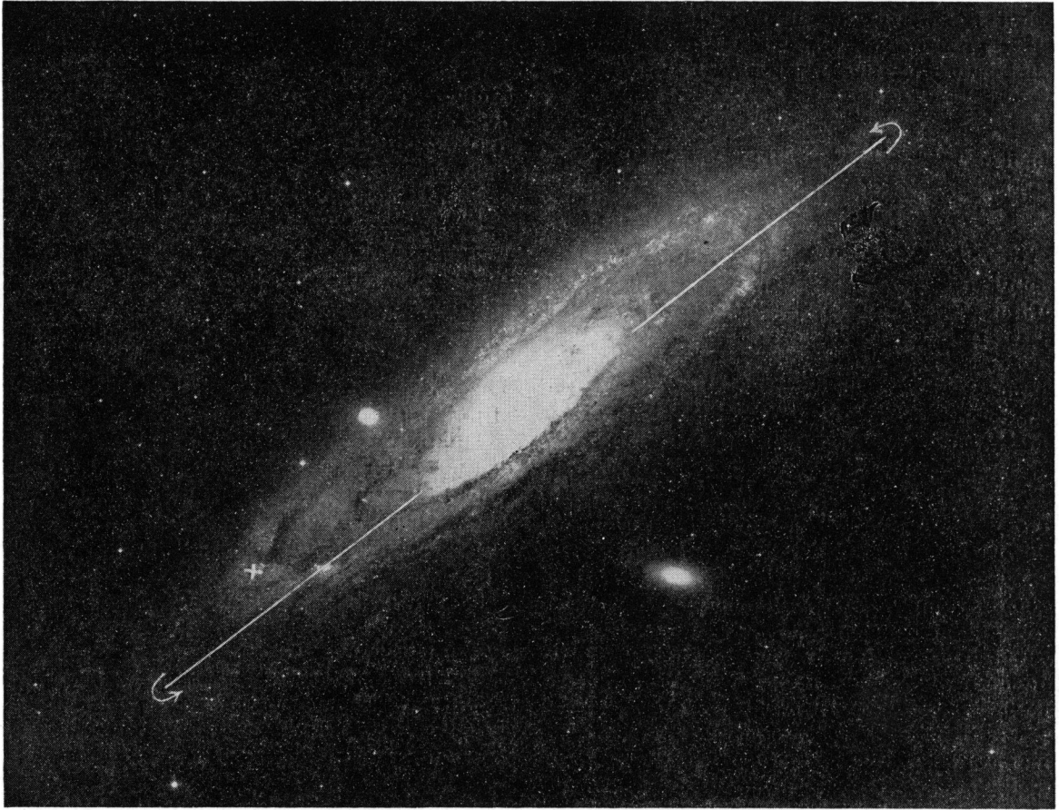
Figure 5. Asymmetry in form of the Andromeda nebula. The sense of the rotation is toward the observer at the lower left, south preceding, and away from the observer at the upper right, north following. The forward motion at the lower left is somewhat slower than the backward motion at the upper right. The major axis is drawn, according to Dr. Baade, through the nucleus, through all the arms at the upper right, and through the outermost arms at the lower left. The perturbed area, marked by a cross, is noticeable by its asymmetric form relative to the major axis. This perturbation may be caused by the close companion, M 32 (to the left of the axis).
