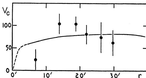
Figure 3. Circular velocity in the spiral galaxy M33. Dots: normal points listed by Mayall and Aller. Vertical lines: probable errors. Curve: computed under assumption of identical mass and light distributions.
