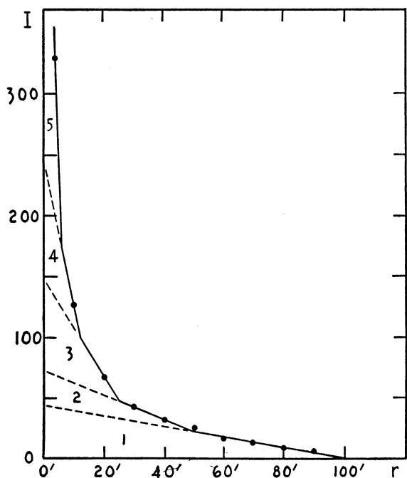
Figure 2. Surface brightness in the Andromeda nebula as represented by straight sections. The dots give the observations by Redman and Shirley as reduced by Wyse and Mayall.
